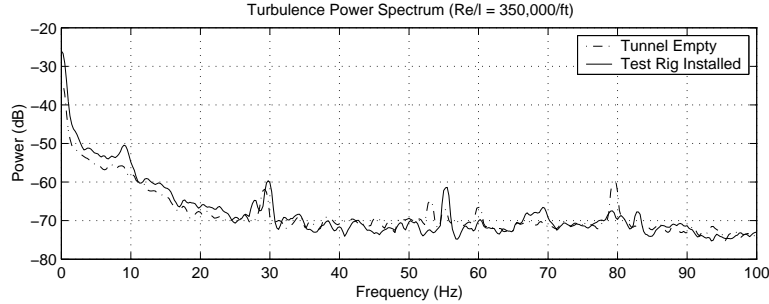
Figure 6. Power spectrum comparison between empty tunnel and installed test apparatus cases for Re = 350,000 .
