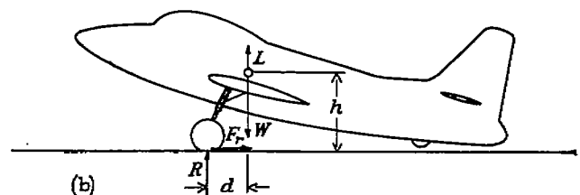
(a) Tricycle landing gear. (b) Conventional landing gear.
