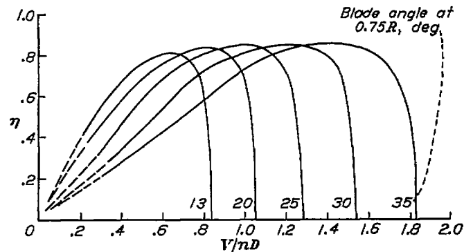
FIGURE 44.—Typical charts showing propeller characteristics.
