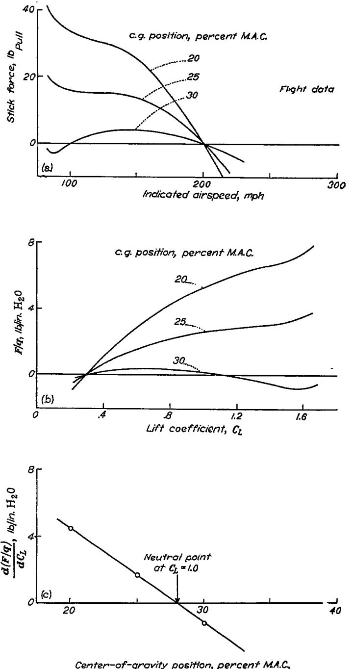
FIGURE 11.—Method for determining stick-free neutral point from flight data.
