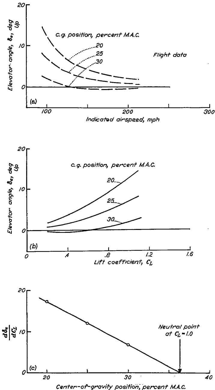
FIGURE 10.—Method for determining stick-fixed neutral point from flight data.
