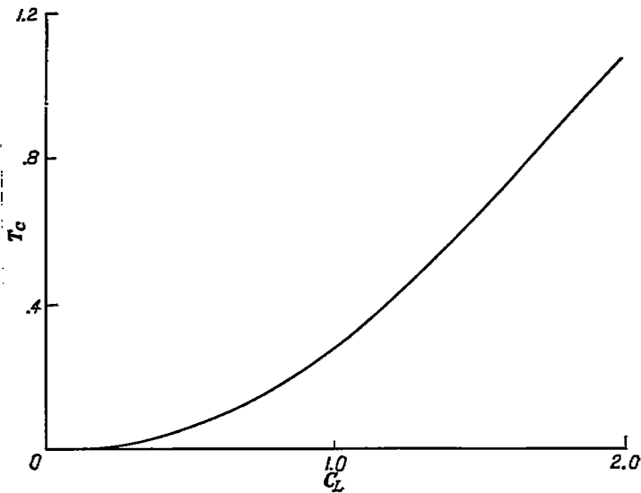
FIGURE 3.—Typical variation of propeller thrust coefficient T_c with lift coefficient in steady flight. T_c = \frac{T}{\rho V^2 D^4} .
