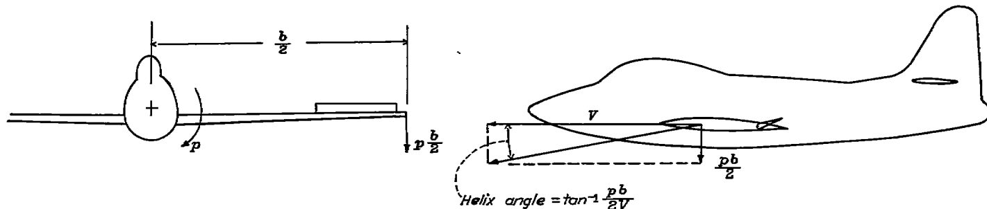
FIGURE 36.—Derivation of the formula for helix angle.
