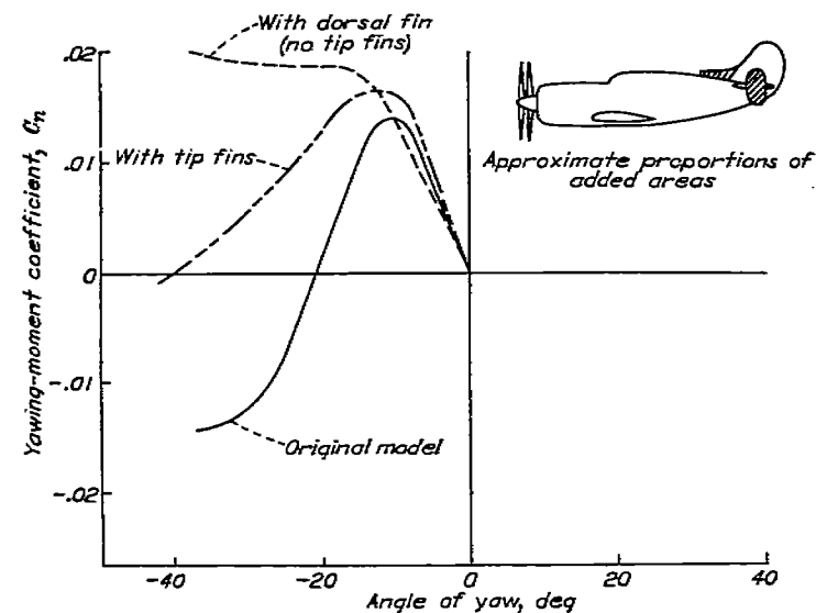
FIGURE 33.—Wind-tunnel measurements showing effect on the directional stability characteristics of a dorsal fin and of vertical fins on the tip of the horizontal tail of a single-engine fighter airplane. Power-on condition (contrarotating propellers); rudder free.
