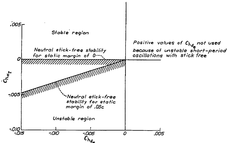
FIGURE 8.—Boundary between stable and unstable values of C_{h_{aT}} and C_{h_{\delta_e}} for the example given in the text. Unstable side of boundaries indicated by cross-hatching.
