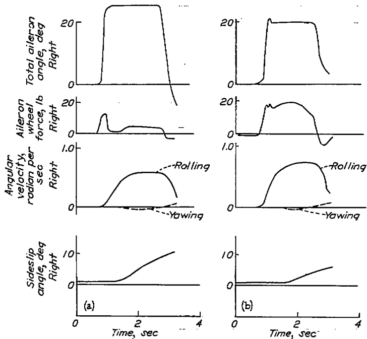
FIGURE 37.—Time histories of typical rudder-fixed aileron rolls in a medium-bomber airplane.
