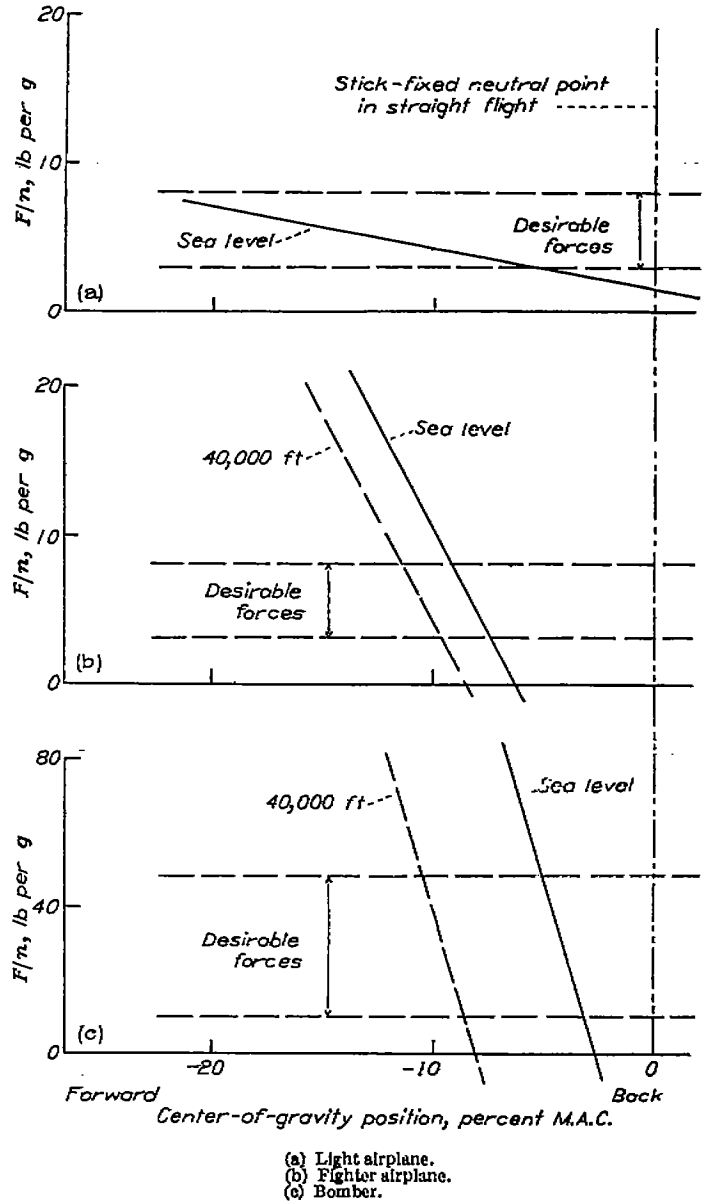
(a) Light airplane. (b) Fighter airplane. (c) Bomber. FIGURE 18.—Stick-force characteristics in maneuvers for three types of airplanes with unbalanced elevators; airplane characteristics given in table I. C_{h_{\alpha}} = -0.003 per degree; C_{h_{\delta}} = -0.007 per degree.
