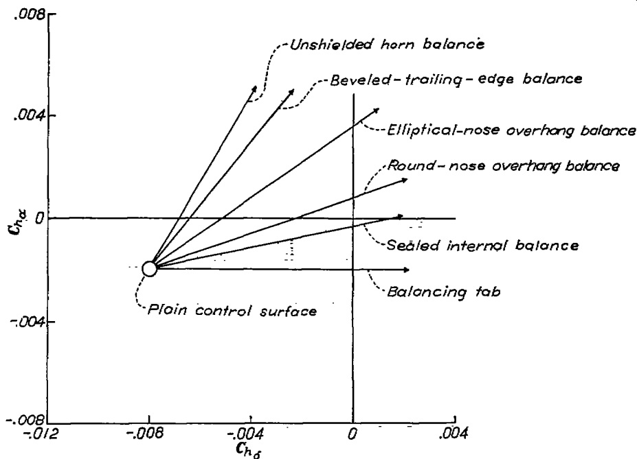
FIGURE 28.—Comparison of effects of various aerodynamic balances on hinge-moment parameters of typical control surface.
