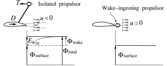
Fig. 7 Comparison of dissipation in isolated and wake-ingesting propulsors for 2D airfoil.
