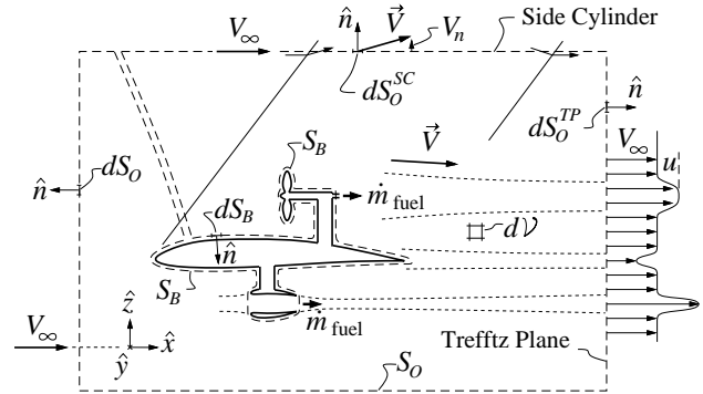
Fig. 1 2D cutaway view of 3D Control Volume surrounding an aerodynamic body. The inner boundary \mathcal{S}_B lies on the body, and may cover moving elements (top propulsor), or hide them inside (bottom propulsor). Vortex-wake velocities v, w on Trefftz Plane are not shown.
