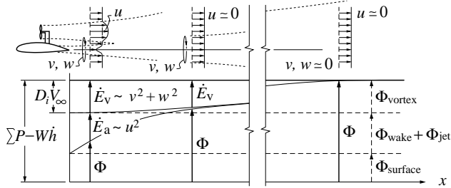
Fig. 4 Variation in power balance terms in equation (37), versus position of Trefftz Plane. Transverse velocities of trailing vortices diffuse much later than the axial velocities of propulsors and wakes. Total dissipated power sum is unchanged. The potential-nearfield contributions to \dot{E}_a, \dot{E}_v are excluded, \dot{E}_p is not shown, and \dot{E}_w is assumed to be zero.
