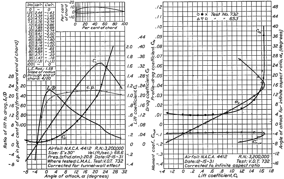
FIGURE 39.—N.A.C.A. 4412 airfoil.
