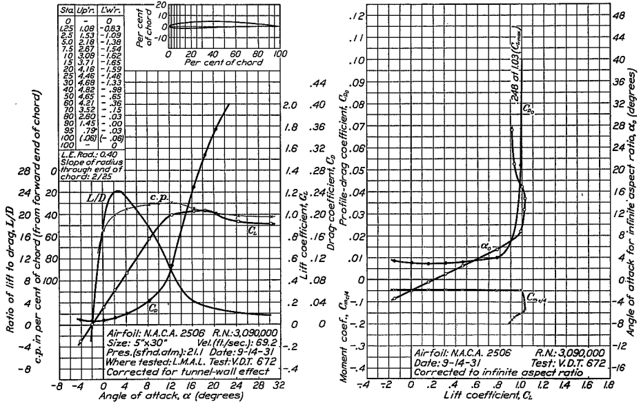
FIGURE 22.—N.A.C.A. 2506 airfoil.
