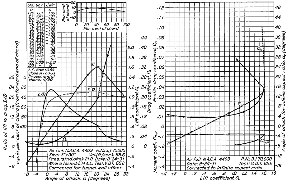
FIGURE 38.—N.A.C.A. 4409 airfoil.
