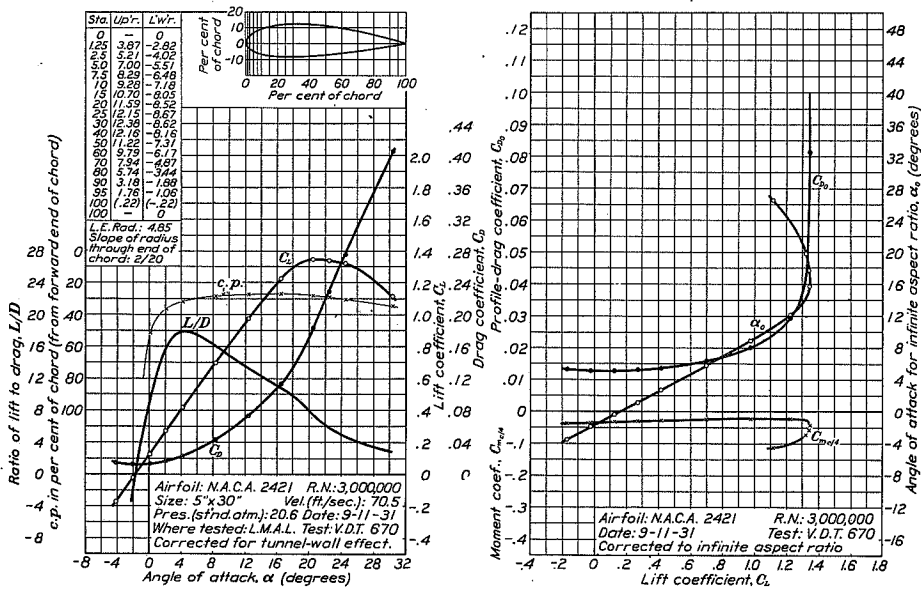
FIGURE 21.—N.A.C.A. 2421 airfoil.
