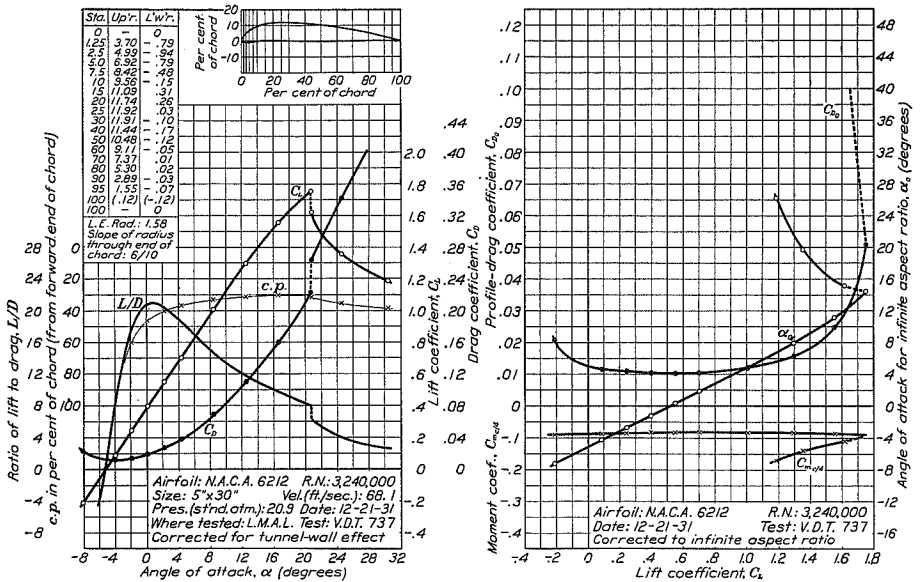
FIGURE 51.—N.A.C.A. 6212 airfoil.
