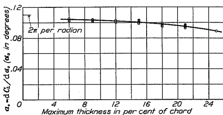
FIGURE 81.—Variation of lift-curve slope with thickness.
