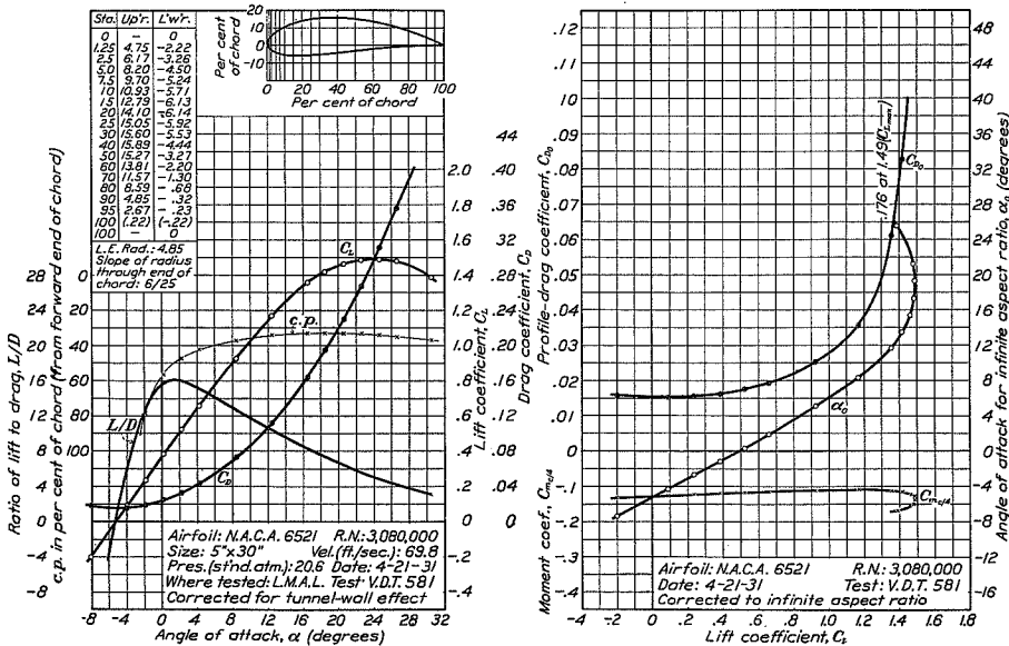
FIGURE 66.—N.A.C.A. 6521 airfoil.
