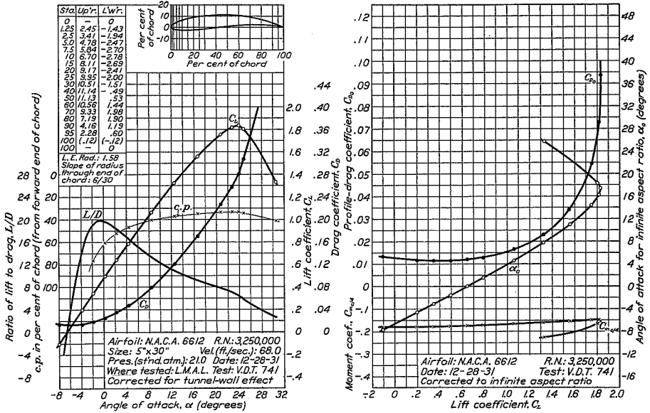
FIGURE 70.—N.A.C.A. 6612 airfoil.
