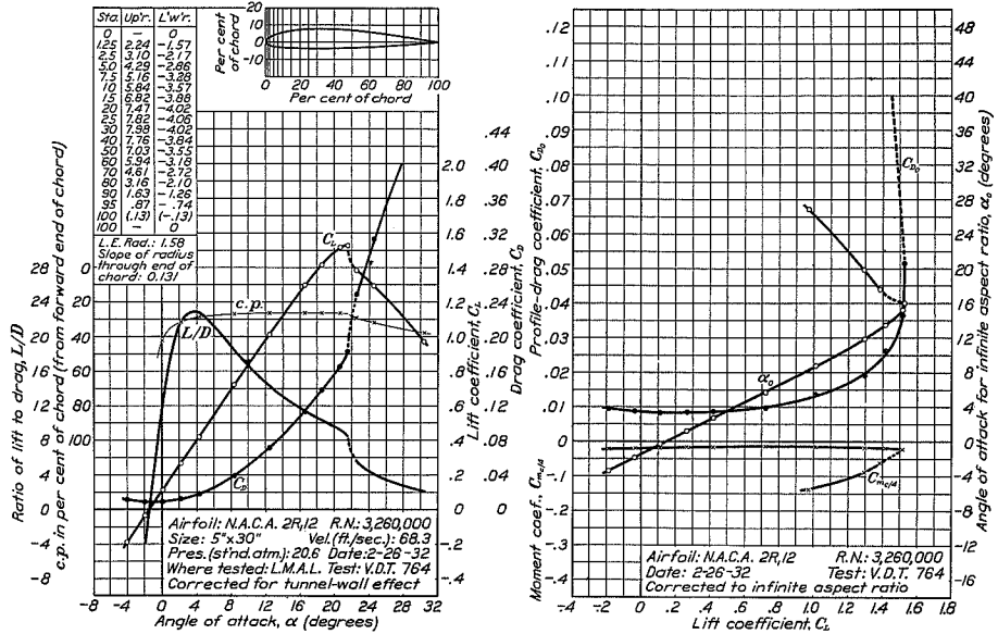
FIGURE 78.—N.A.C.A. 2R 1 12 airfoil.
